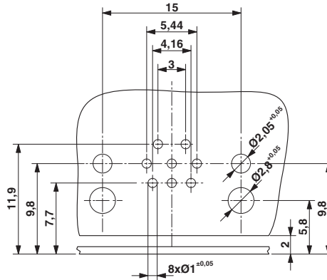
Drilling diagram
